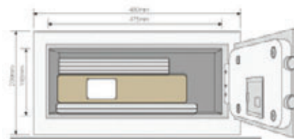
Varenr. 924652 YLB/200/EB1 – Basis laptop
